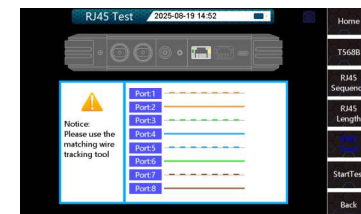
RJ45 Track
