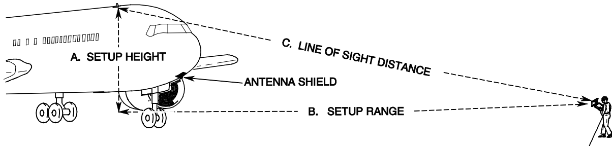
TESTING TOP ANTENNA
