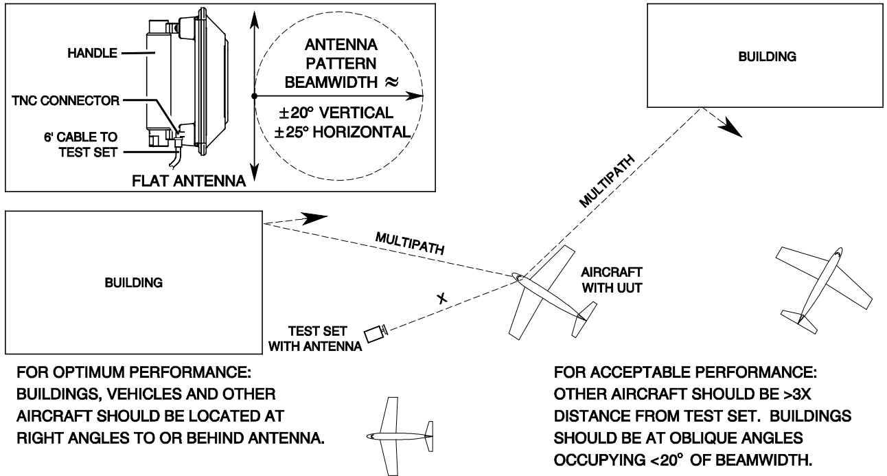
Suggested Layout to Reduce Multipath Errors Figure 11
