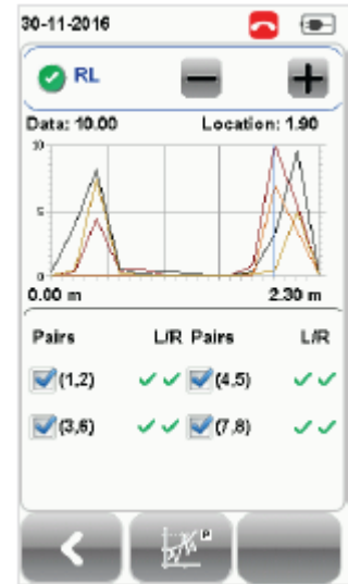
Return Loss Locator
