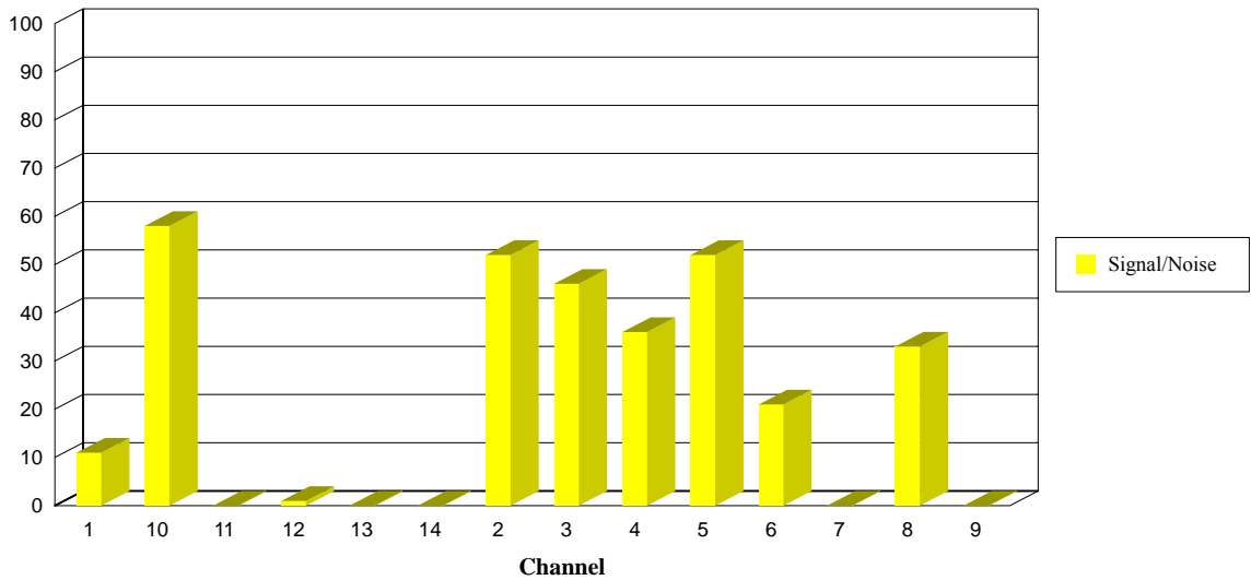
Signal/Noise (2.4 GHz) (%)
